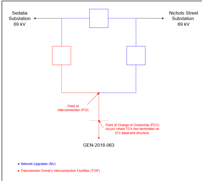
Figure 2 – Preliminary One-Line for new POI substation
